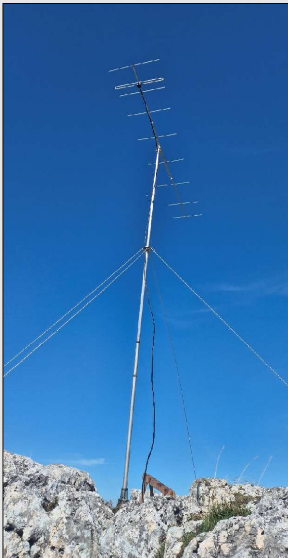
HB9IAB/p – Eric – 9ele on QTH Chasseron (VD) JN36GU
